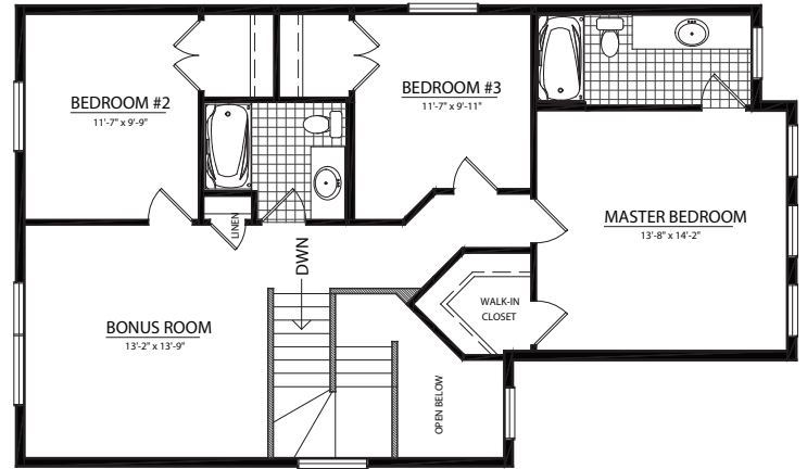
Optional Second Floor A - 985 Sq.Ft.
